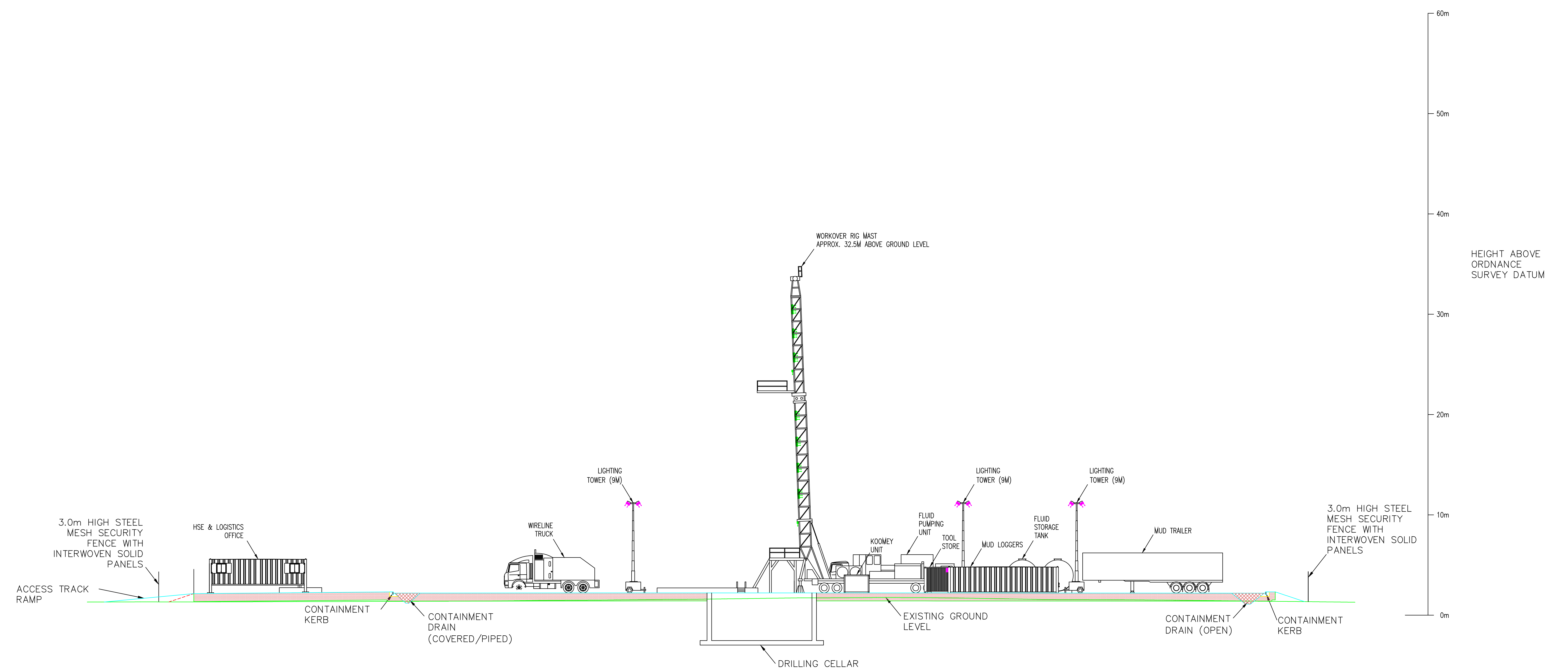
INDICATIVE SECTION N-N THROUGH WELL ABANDONMENT PHASE [1:200]
