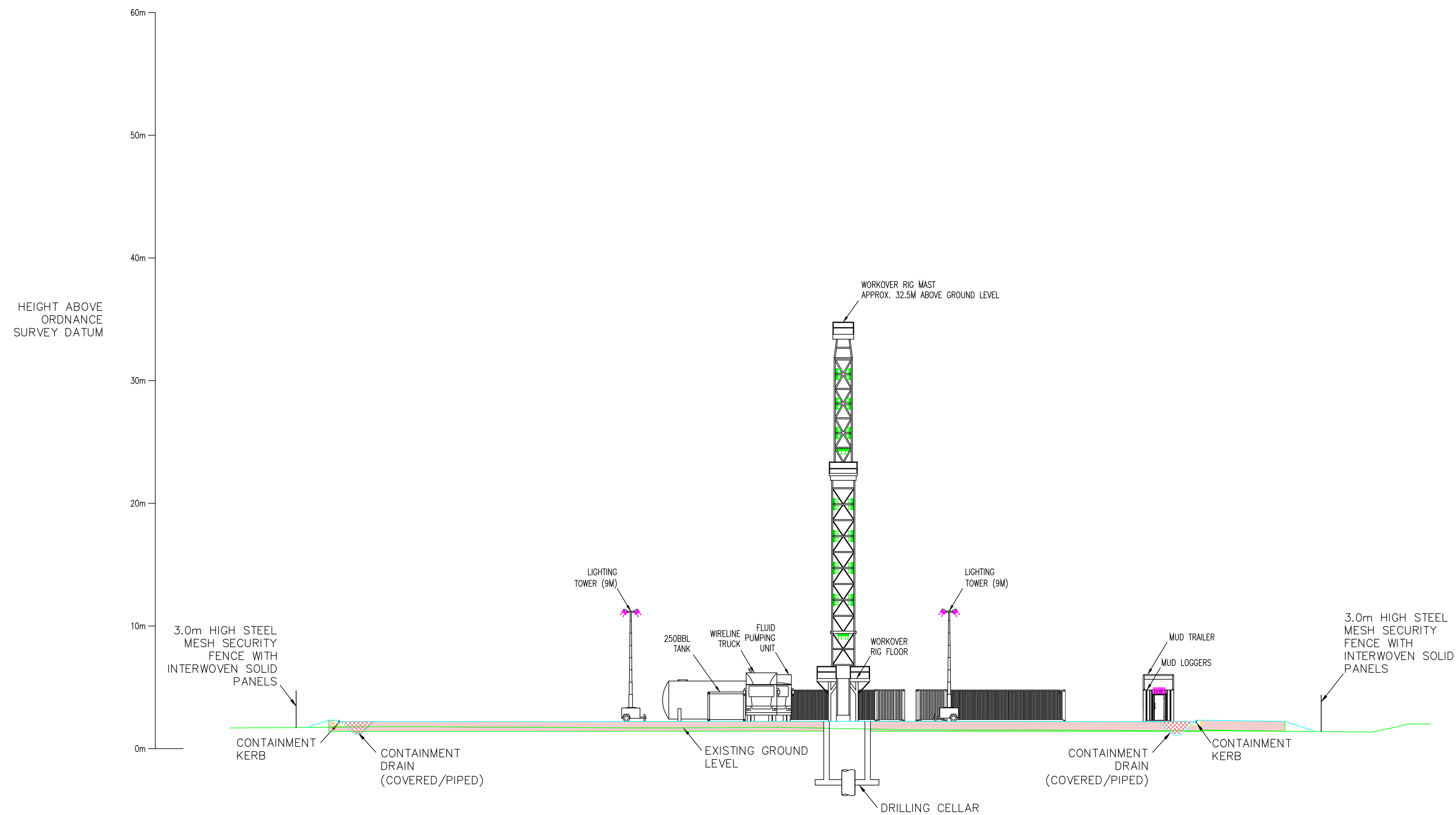
SECTION M-M THROUGH WELL ABANDONMENT PHASE [1:200]
