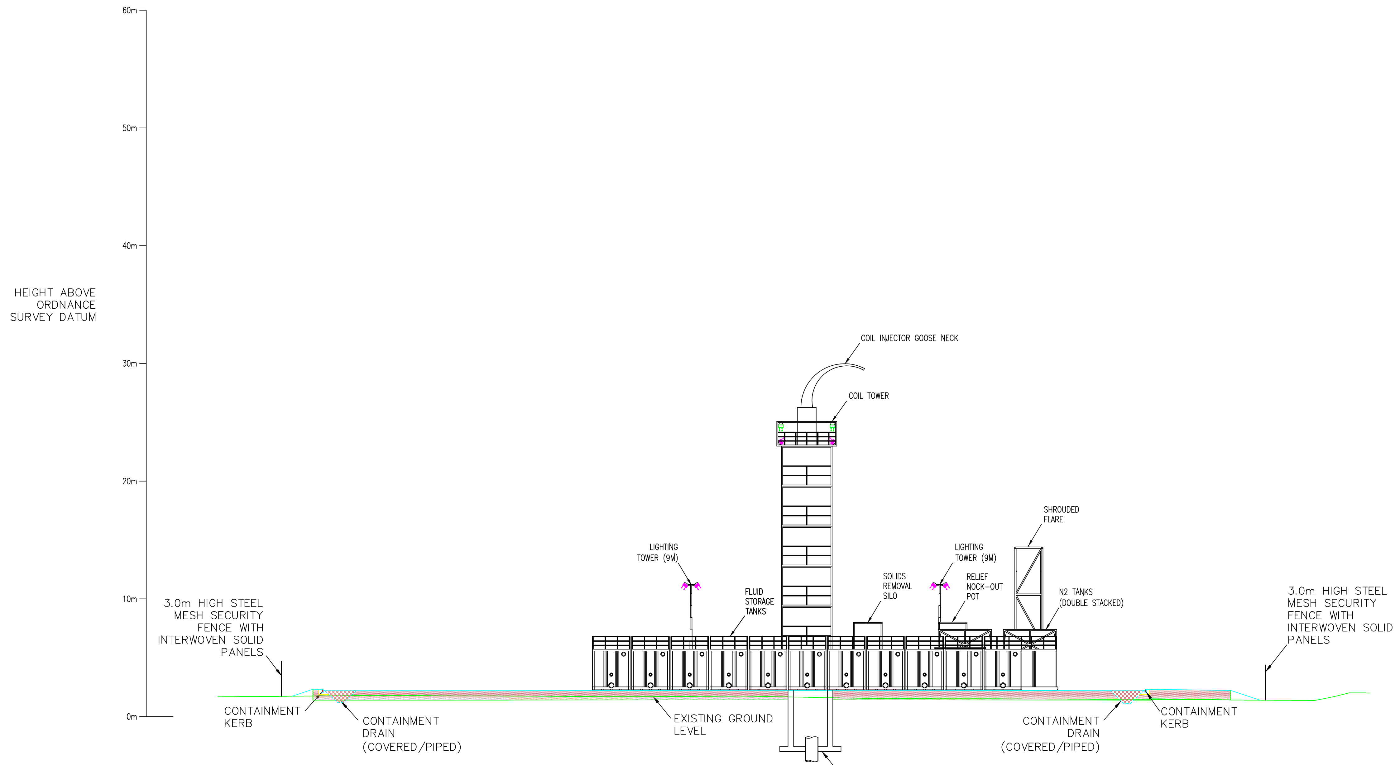
SECTION I-I THROUGH INITIAL FLOW TEST PHASE [1:200]
