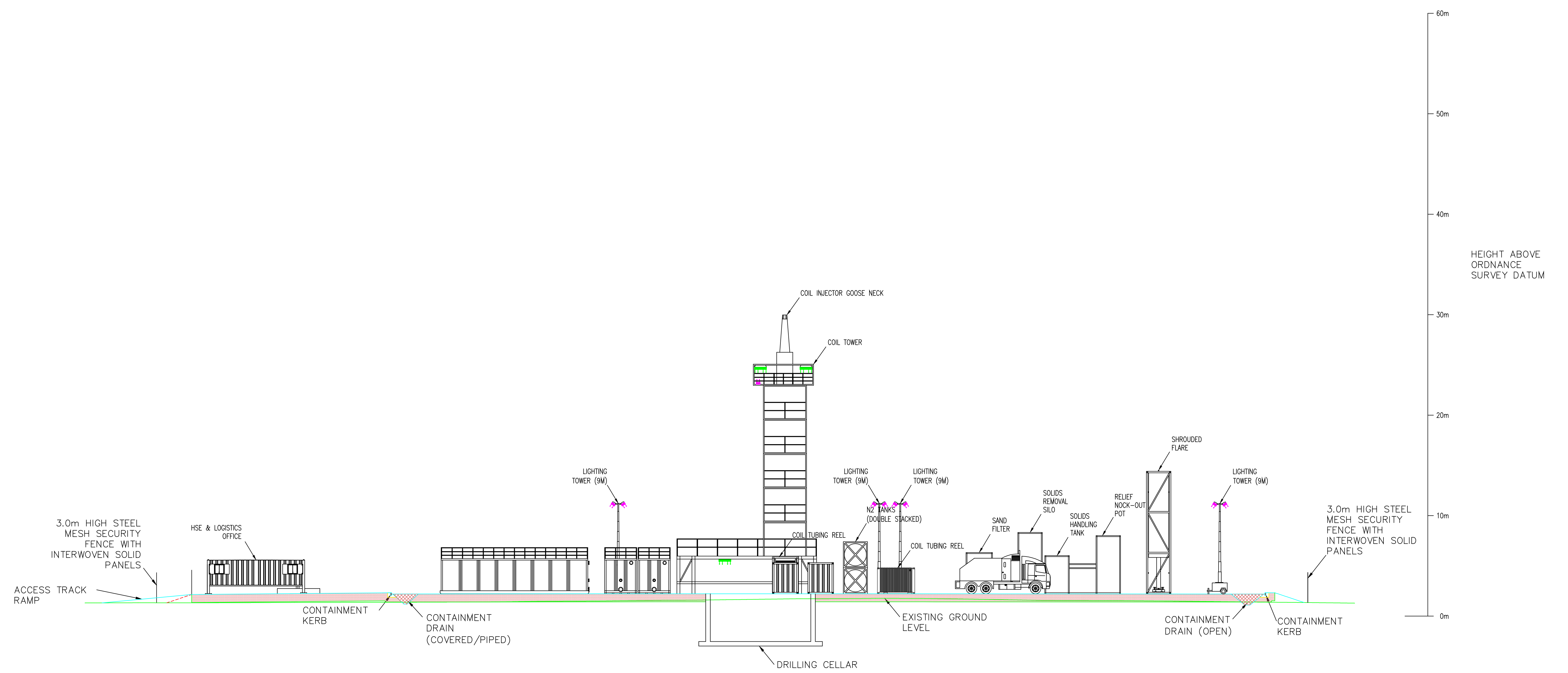
INDICATIVE SECTION J-J THROUGH INITIAL FLOW TEST PHASE [1:200]
