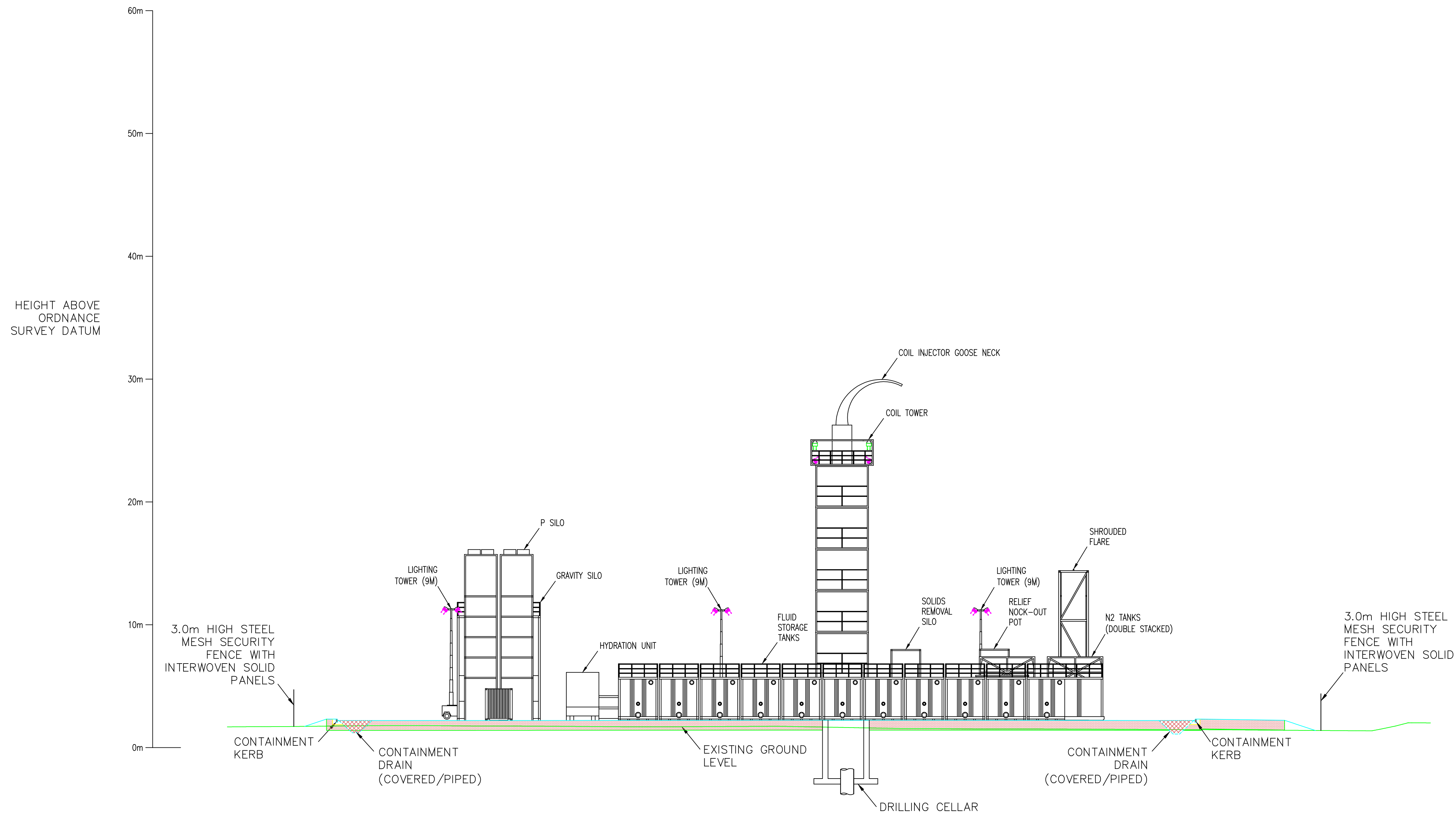
SECTION G-G THROUGH HYDRAULIC FRACTURING PHASE [1:200]
