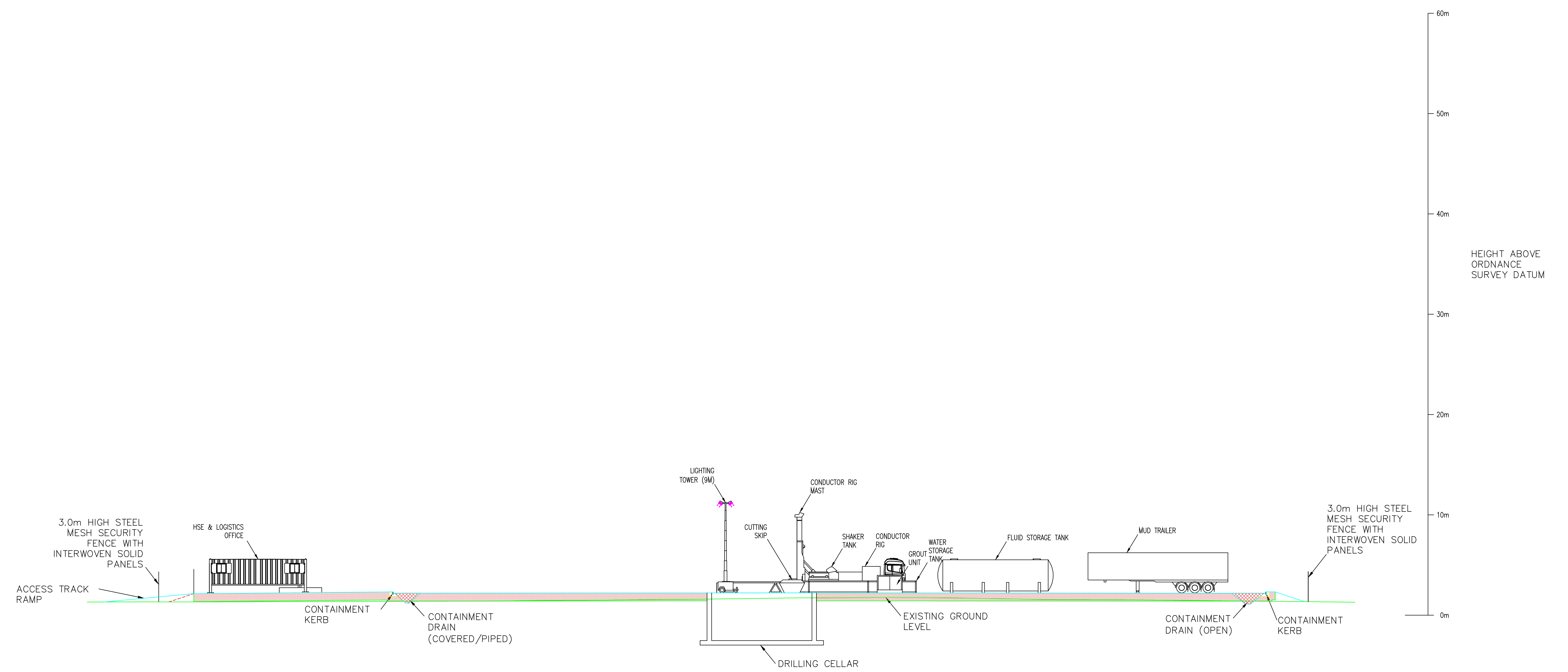
INDICATIVE SECTION D-D THROUGH CONDUCTOR SETTING PHASE [1:200]
