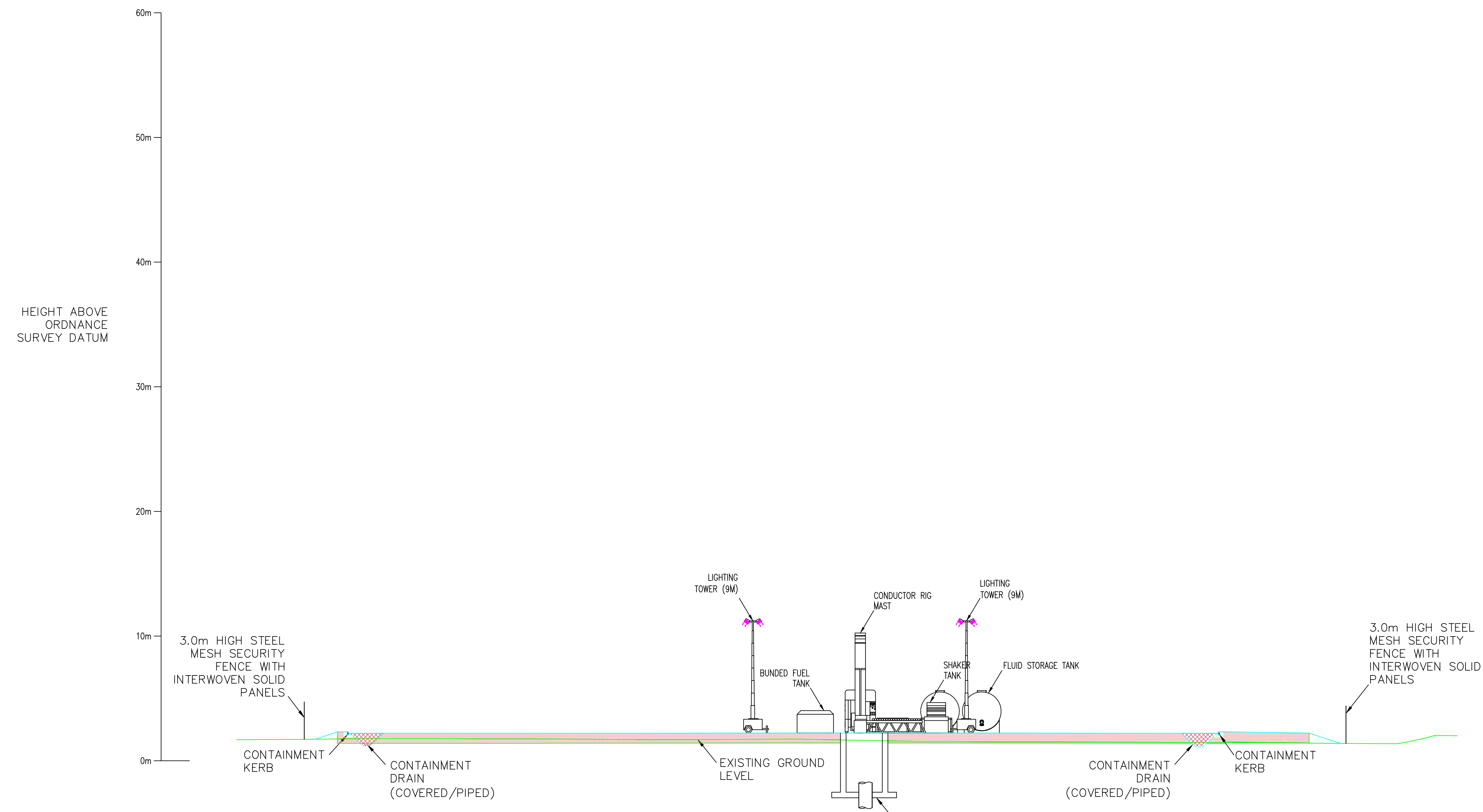
SECTION C-C THROUGH CONDUCTOR SETTING PHASE [1:200]
